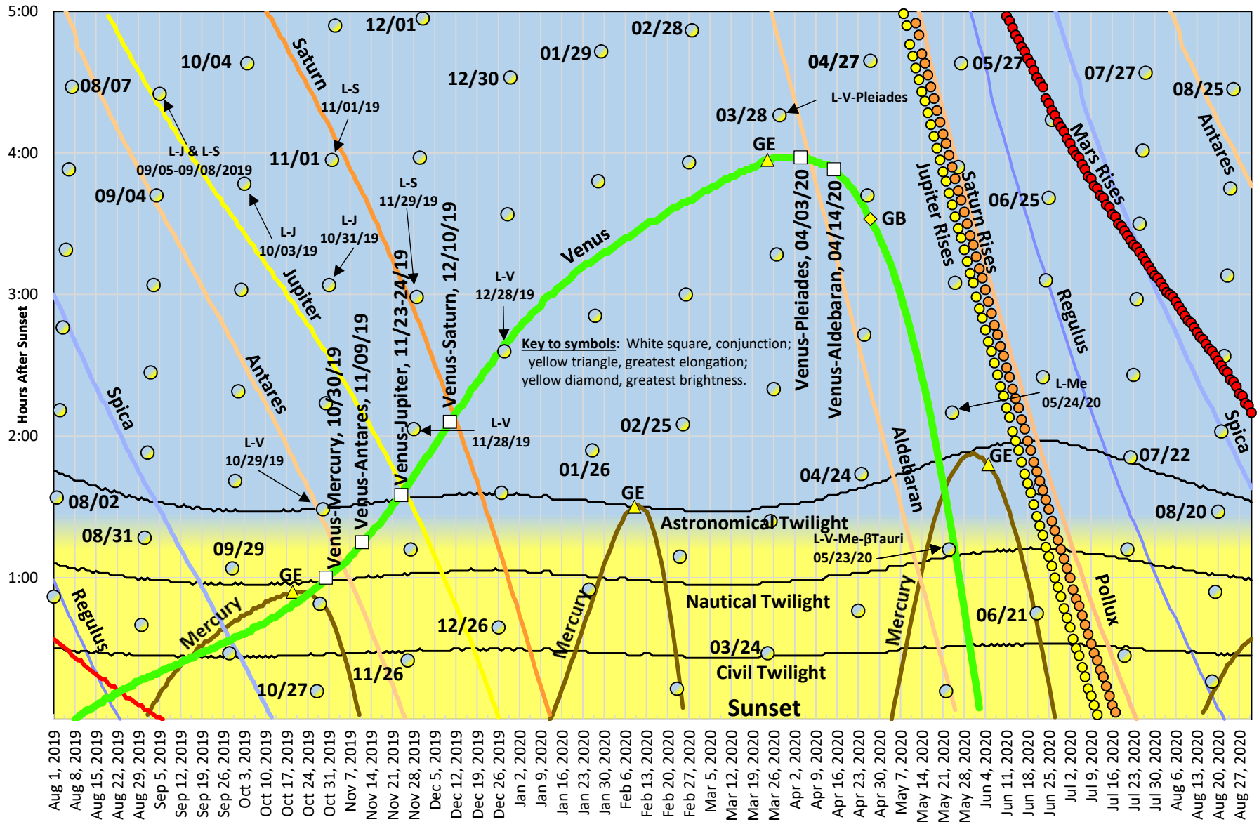
All moon dots, and the curves for planets and stars, indicate setting times in relation to sunset, except for the three planets' curves labeled to indicate times of rising, also in relation to sunset.
