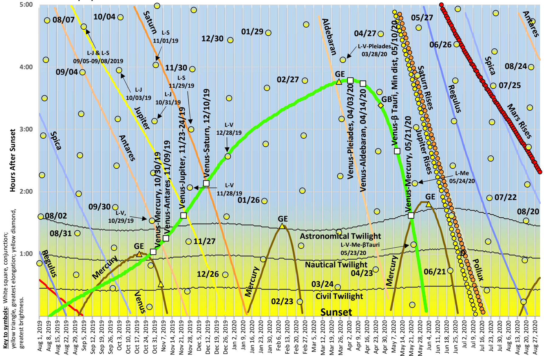
All Moon dots, and the curves for planets and stars, indicate setting times in relation to sunset, except for the three planets' curves labeled to indicate times of rising, also in relation to sunset.
